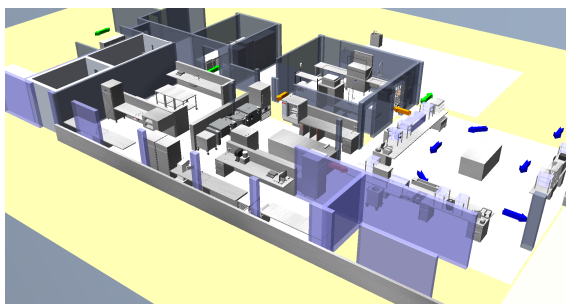
3D-Modell
